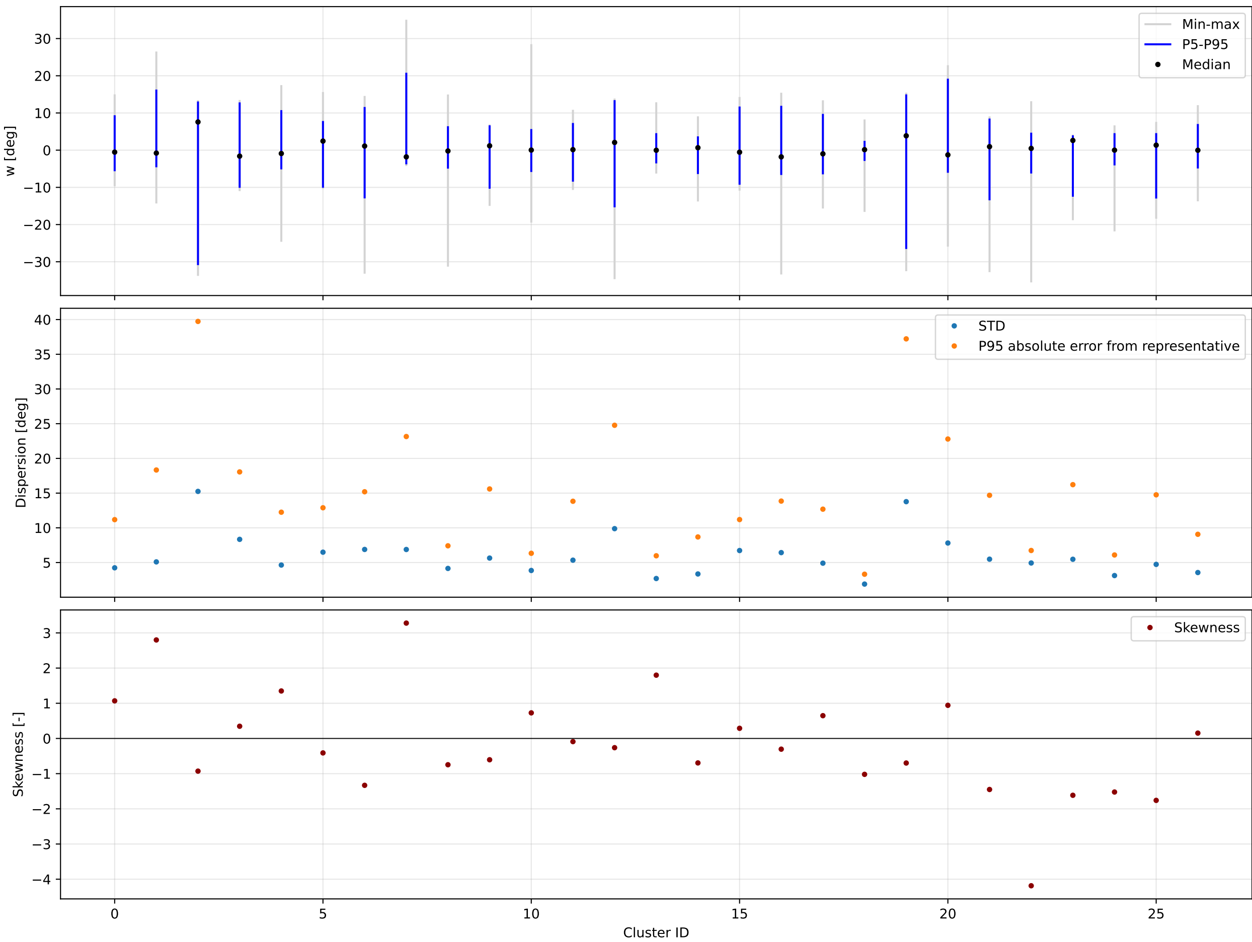
K=27 | backward | w | valid=194124/194124 | offsets from each cluster circular mean
